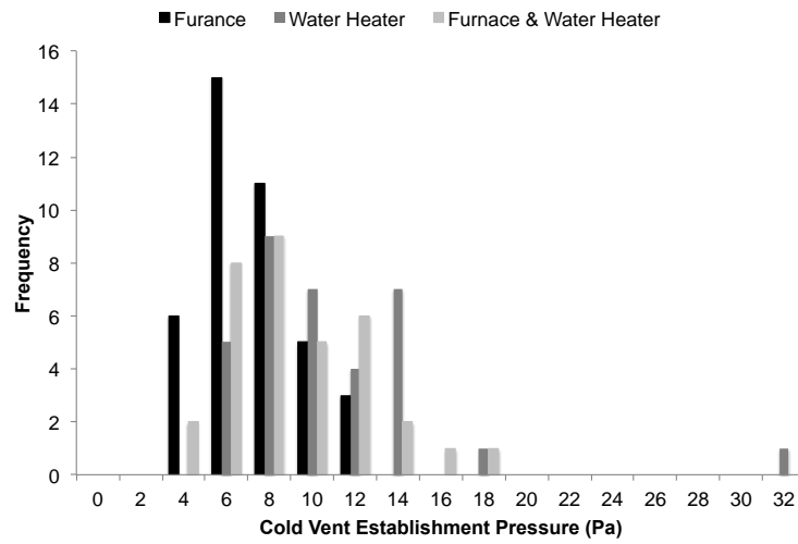
Figure 1: Distribution of CVEP for furnaces, water heaters, and furnaces and water heaters operating simultaneously. Data were taken from 40 houses located in Toronto (1988) [55].
