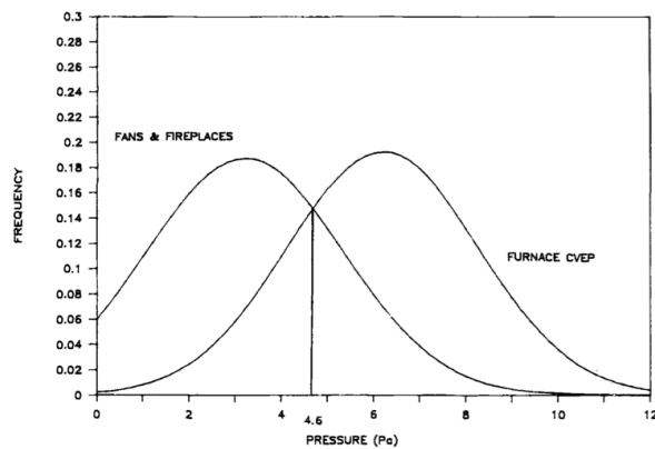
(c) Distribution of furnace CVEP and house depressurization from operating exhaust fans and fireplace. Mean depressurization from fans and fireplace = 3.16 Pa, standard deviation = 2.08 Pa, mean furnace CVEP = 6.2 Pa, standard deviation = 2.08 Pa. Probability of one random reading being under both normal curves simultaneously = 23%.
