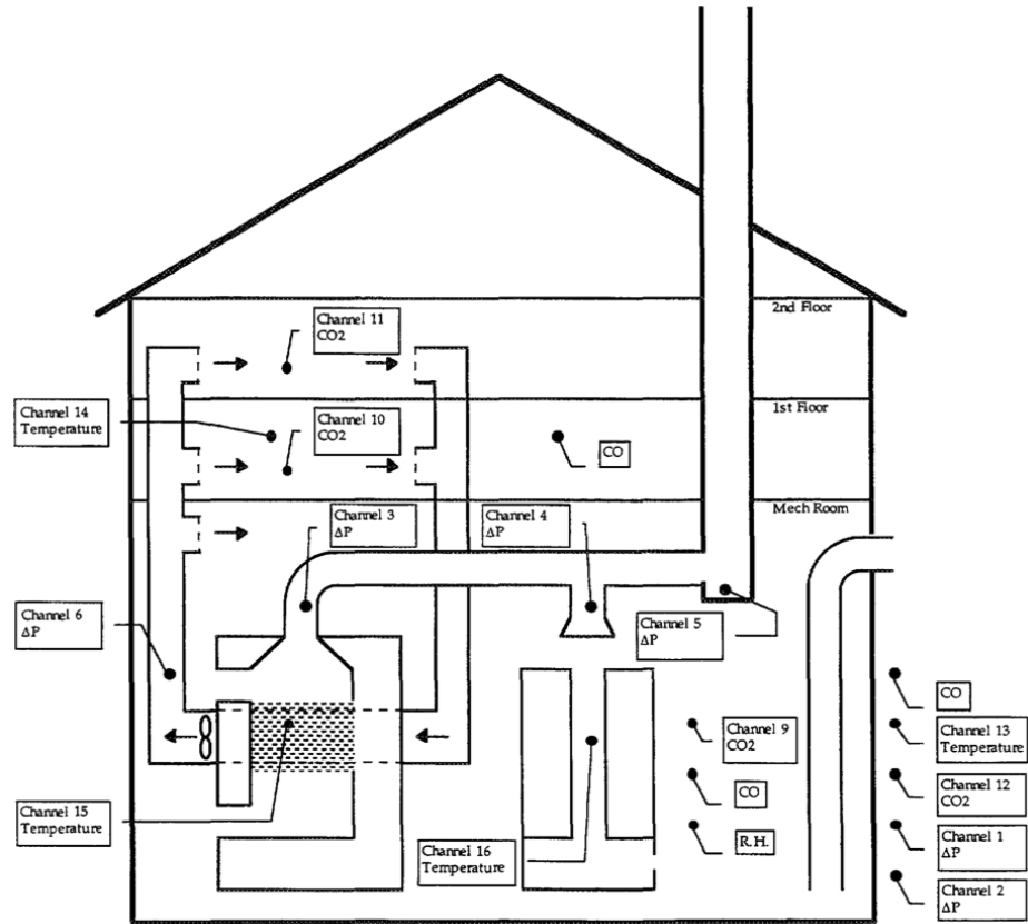
Figure 4: Grimsrud et al. [25] house measurements and measurement locations for homes in Minnesota and Chicago
