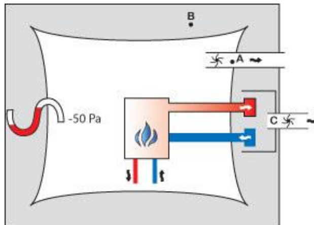
Figure 6: Simplified concept of depressurization spillage test taken from the report [16]
