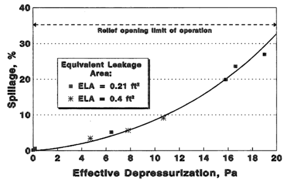
Figure 5: Correlations between spillage and effective depressurization for induced draft and natural draft combustion appliances tested in AGA Research House (1996) [5]
